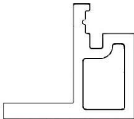
Starting/finishing Slatted Cladding F-type Trim 36,5 x 56 mm
