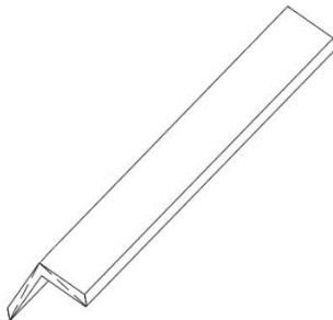
Starting/finishing Slatted Cladding F-type Trim 36,5 x 56 mm
