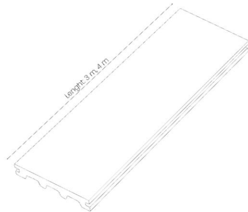
SOLID PREMIUM DECKING BOARD 23 x 138 mm
